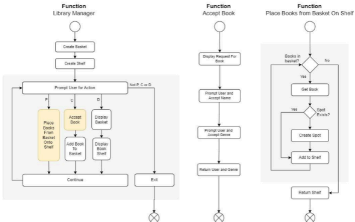
Figure 1: Behavioral semantics of the library manager.
